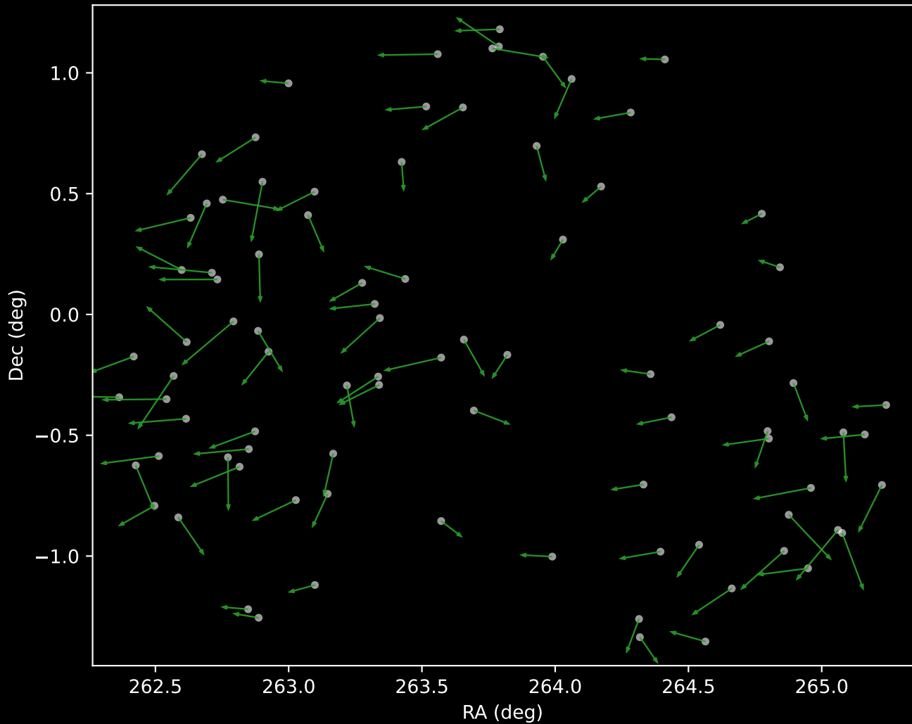
APOGEE DR17 Cluster 4 Proper Motion Vectors (n=89)
