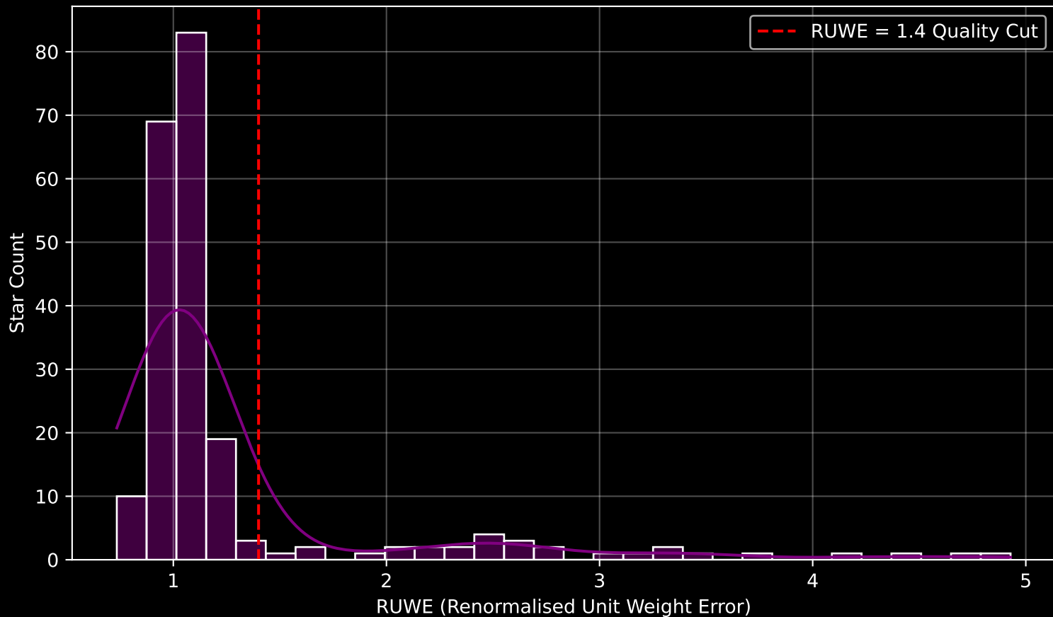
GAPOGEE DR17 Field [253+51] RUWE Distribution (n= 213)
