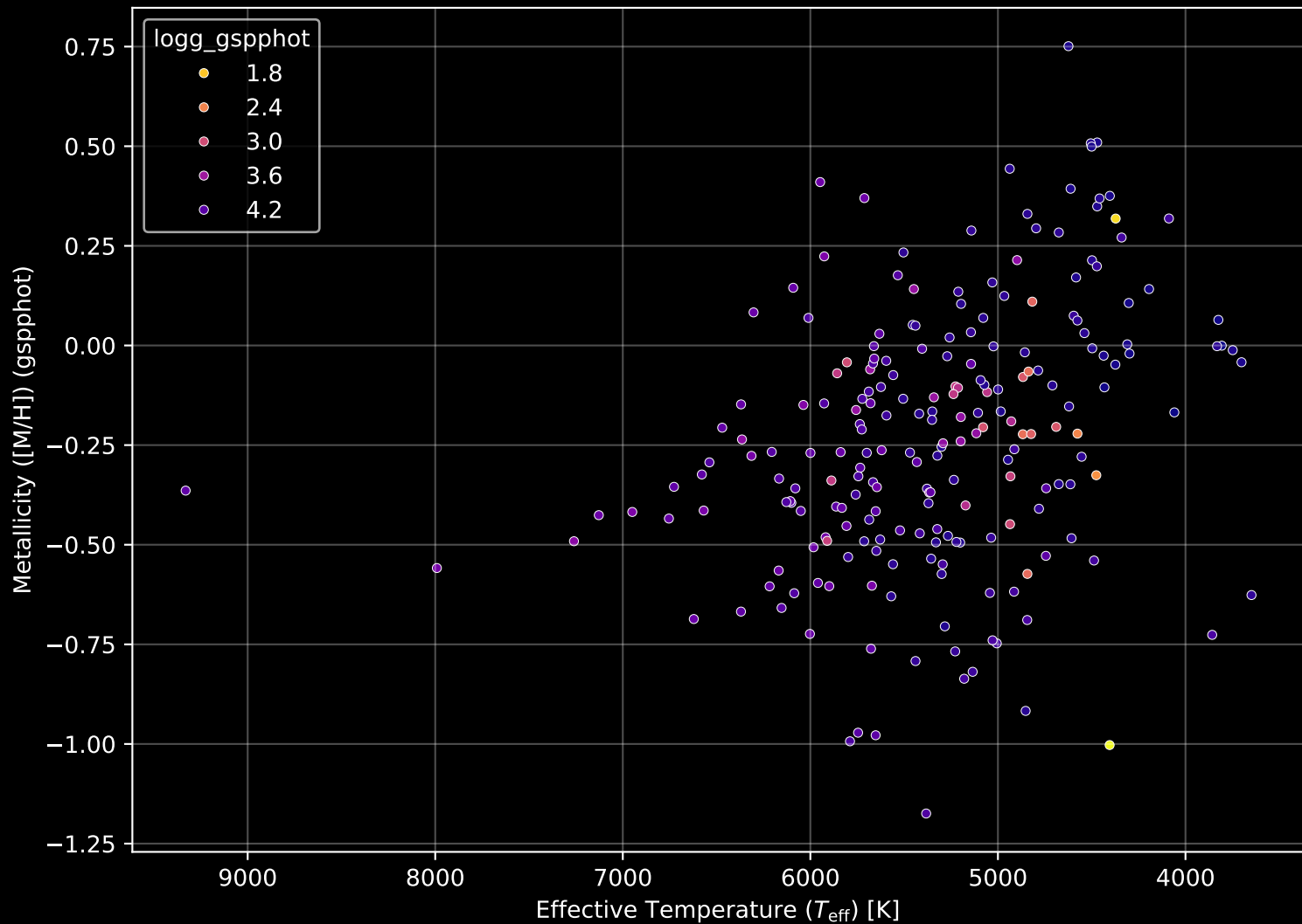
APOGEE DR17 Field: [253+51] Stellar Population Parameters (n= 218)
