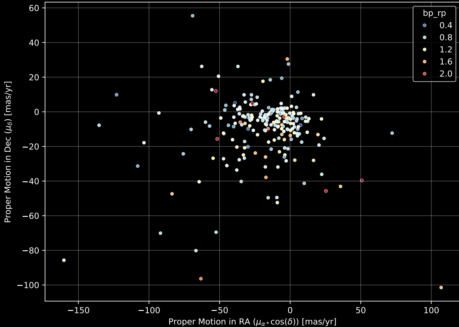
APOGEE DR17 Field: [253+51] Proper Motion Diagram (n= 218)
