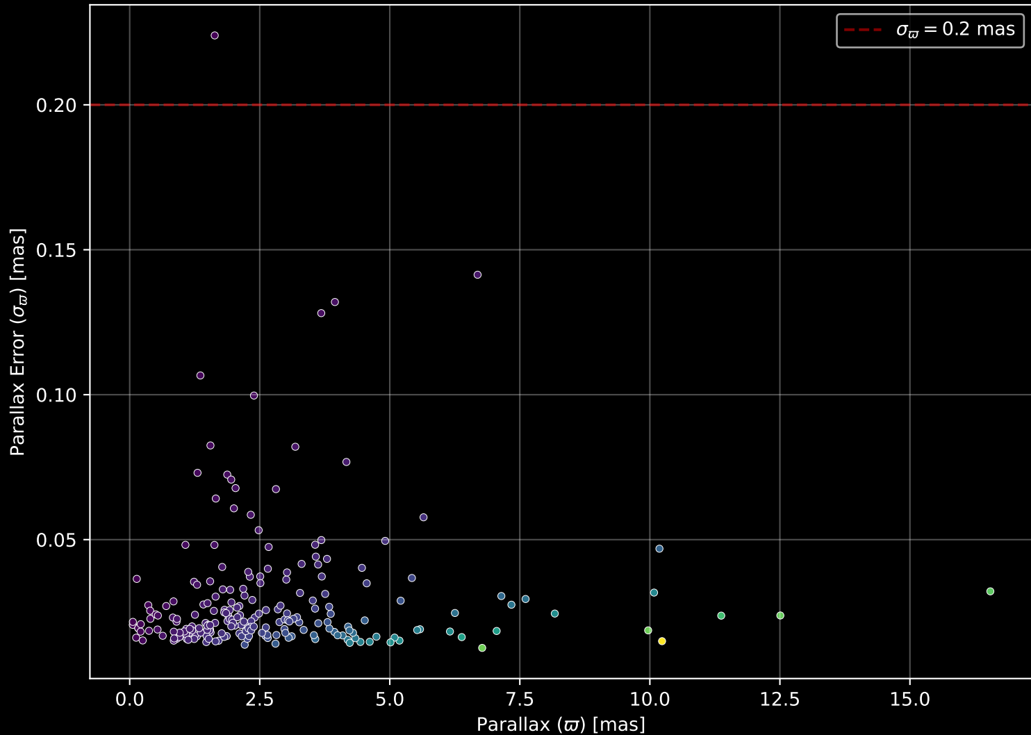
APOGEE DR17 Field: [253+51] Parallax Quality (n= 218)
