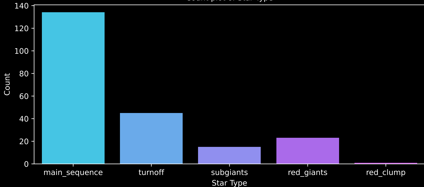
APOGEE DR17 Field: [253+51] Count plot of Star Type
